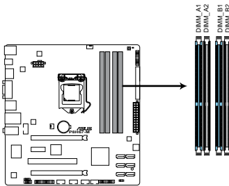
P8H67-M 240-pin DDR3 DIMM sockets
