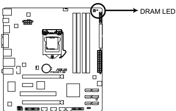
P8H67-M DRAM LED
