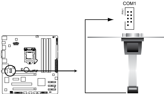
P8H67-M Serial port (COM1) connector
