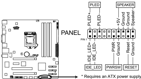
P8H67-M System panel connector
