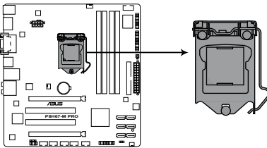
P8H67-M CPU socket LGA1155
