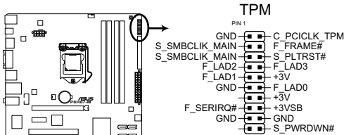
P8H67-M TPM Connector
