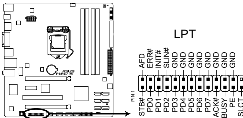
P8H67-M Parallel Port Connector
