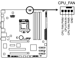
P8H67-M CPU fan connector
