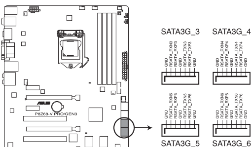
P8Z68-V PRO/GEN3 Intel® SATA 3.0 Gb/s connectors
