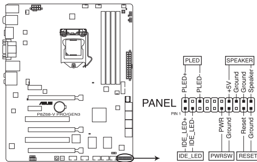
P8Z68-V PRO/GEN3 System panel connector
