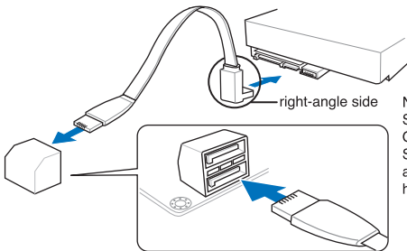
P8Z68-V PRO/GEN3 Intel® SATA 6.0 Gb/s connectors
